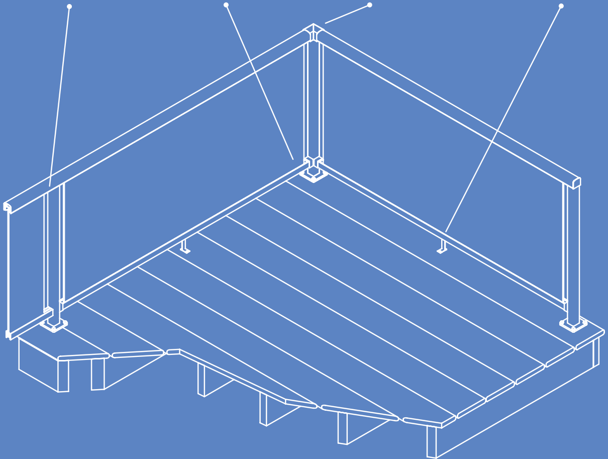
leg support
