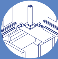
bottom detail
